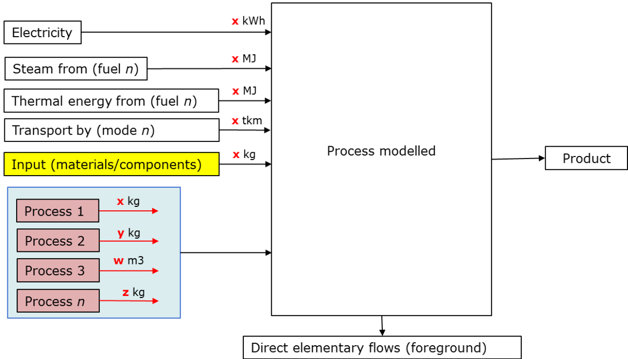
5704 Figure 12: Minimum level of disaggregation requested for a dataset aggregated at level 1. The yellow box is 5705 optional when going beyond the minimum requirements.
