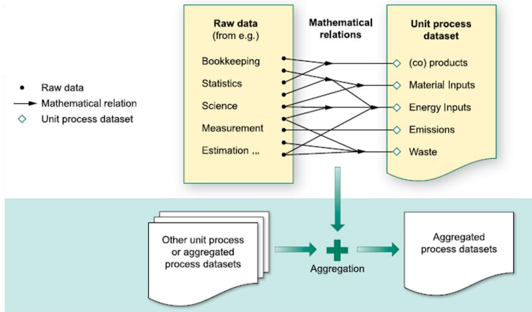
473 474 Figure 1: Definition of a unit process dataset and an aggregated process dataset
