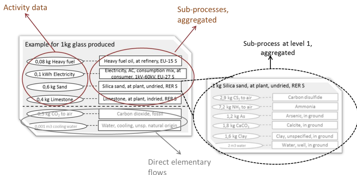
551 552 Figure 2: An example of a partially disaggregated dataset, at level 1. The activity data and direct 553 elementary flows are to the left, and the complementing sub-processes in their aggregated form are to the 554 right. The grey text indicates elementary flows
